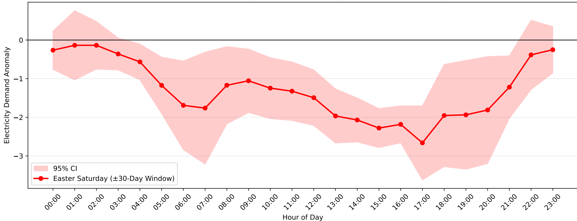
Charmhaven Demand Anomaly: Easter Saturday (2004–2017, \pm 30 -Day Window)
